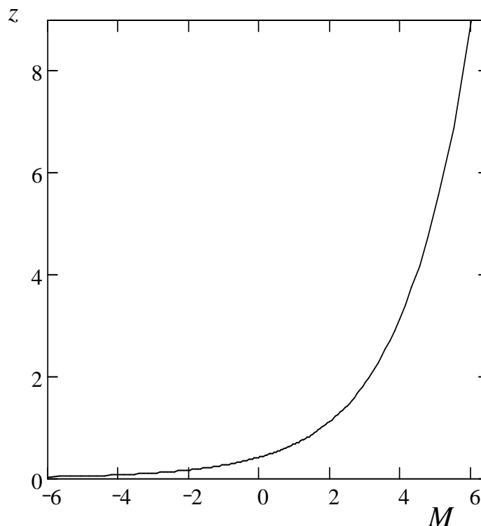
Fig. 7. Dependence z on M . For large z the brightness of stars, quasars and galaxies is weakly dependent in z , since near the particles horizon small variations in distance from the source corresponds to a large range of changes in z .
