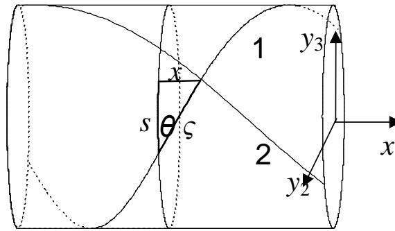
Fig. 3. 1 – helical trajectory of a particle moving in a six-dimensional space with the speed of light on the cylindrical surface of Compton radius \hbar/(mc) with axis in the subspace X and the directrix in the subspace Y ; 2 – helical line intersects the helical trajectory at right angles and passes through the particle. It moves along the tube at the speed of de Broglie waves. Its step is the de Broglie wavelength. This is the line of the same proper time of the particle.
