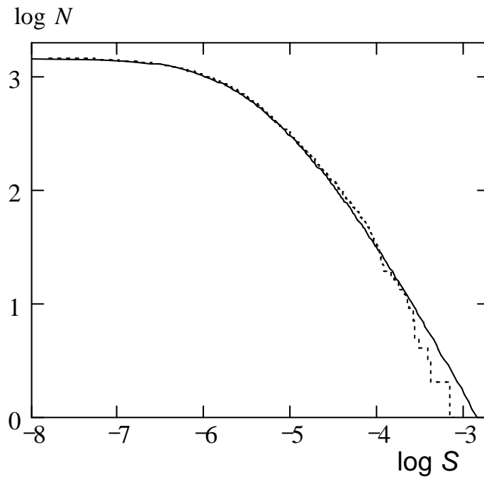
Fig. 10. Logarithm of the distribution function of gamma-ray bursts as a function of the logarithm of the detected energy flux: calculated (solid line) and measured (dotted)
