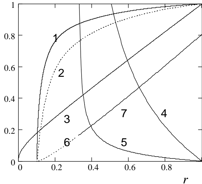
Fig. 6. Depending on r = R_*/R , the relative cosmological time 1 – the relative velocity of light, 2 – its square, 3 – the relative radius of 3D sphere, 4 – redshift z(r) , 5 – z(r)/10 , 6 – relative time by the light clock, 7 – the same closer then the particle horizon.
