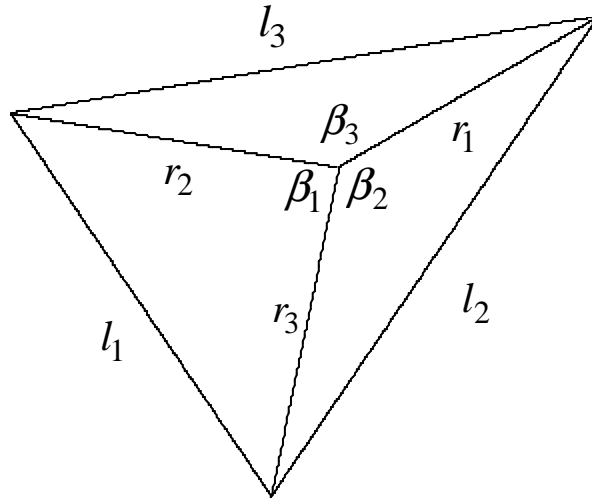
Fig. 4. The radii r_j of three N D spheres in the plane on which the centers of spheres placed when the intersection of all three spheres is at one point. Centers of N D spheres are located at the vertices of the large triangle, l_j the distances between the centers, j = 1, 2, 3 . In the case of the 6D space N = 5 .
