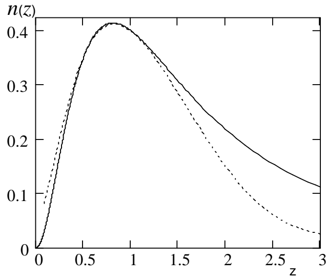
Fig. 9b. The same theoretical curve in comparison with the later experimental curve [56]
