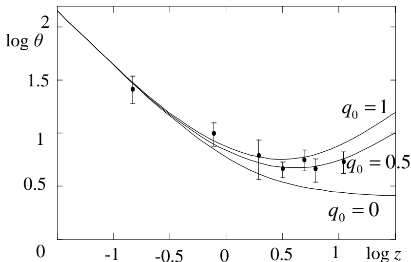
Fig. 2. The dependence of the angular size of the double radio sources (in angular milliseconds) with the linear size of 41 parsecs on redshift z .
