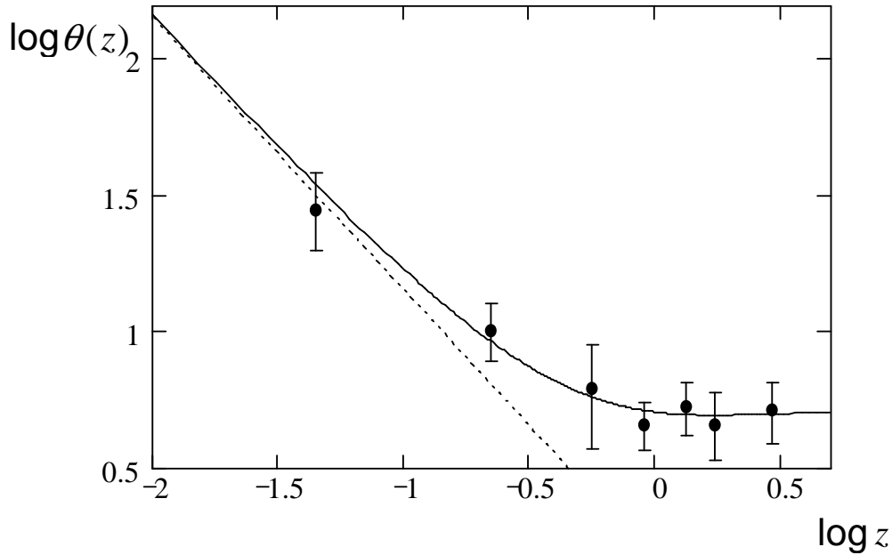
Fig. 8. Dependence on z the angular size (in milliarcseconds) double source having at cosmologically close distances linear size of 41 pc.
