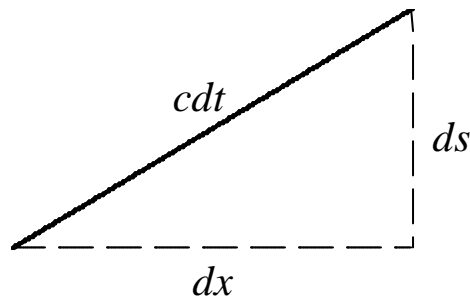
Fig. 1. Projections ds and dx of displacement cdt of a particle moving at the speed of light in the whole space. These three quantities are related to the Pythagorean theorem
