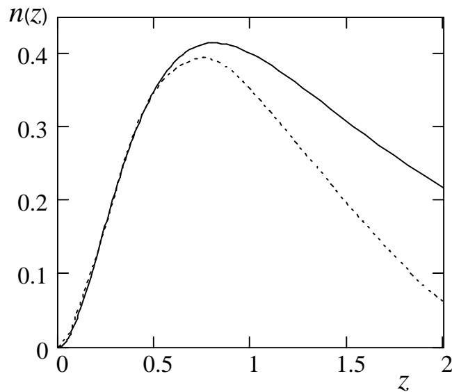
Fig. 9a. Relative density distribution of number of galaxies at redshift z : calculated (solid line) and measured (dashed) [12].
