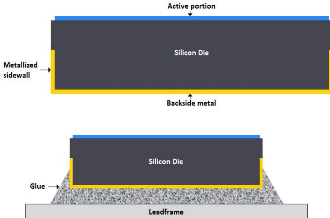
Fig. 2. Advanced semiconductor die construction
