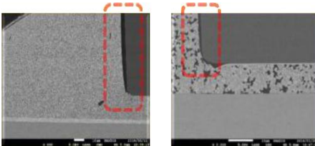
Fig. 1. Cross-sectional view of silicon die interface with glue
