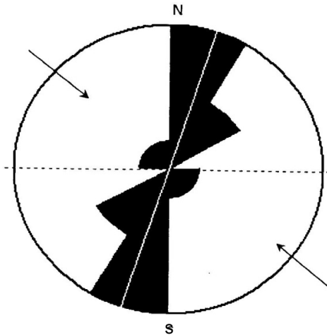
Fig. 12. Above shows a rose diagram indicating the dominant trend of joints on granite exposures veins are tabular or sheet-like bodies which have intruded into the main lithological unit through joints and fissures of various lengths and thickness. Veins observed in the study include quartz and pegmatite veins Fig. 14
