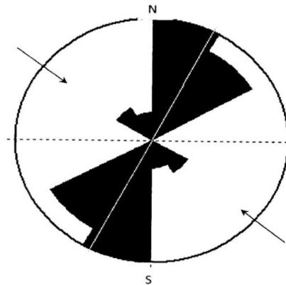
Fig. 13. Above shows a rose diagram indicating the dominant direction of stress on gneiss exposures
