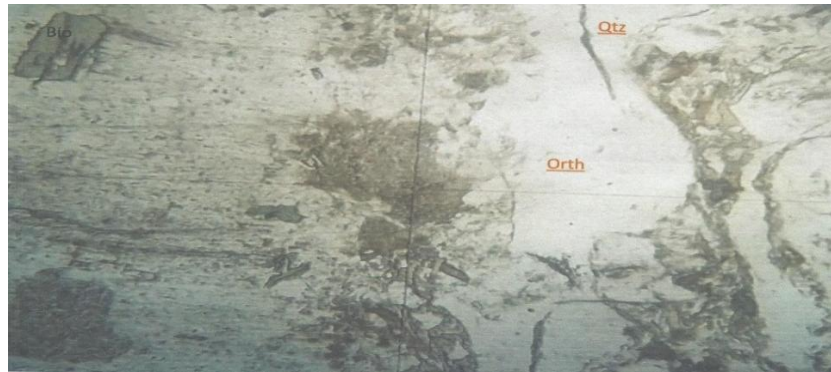
Fig. 10. PPL (X40) Photomicrograph of granite, showing euhedral crystals of orthoclase feldspar and some biotite embedded in the groundmass (Orth-orthoclase, Bio-biotite and Qtz-quartz)
