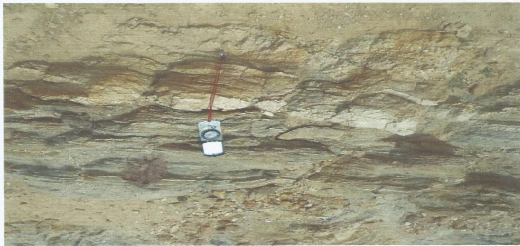
Fig. 3. Field photograph of a highly foliated weathered gneiss along a river channel with coordinates latitude 11°36'26.5"n and longitude 007°31'13.8"e
