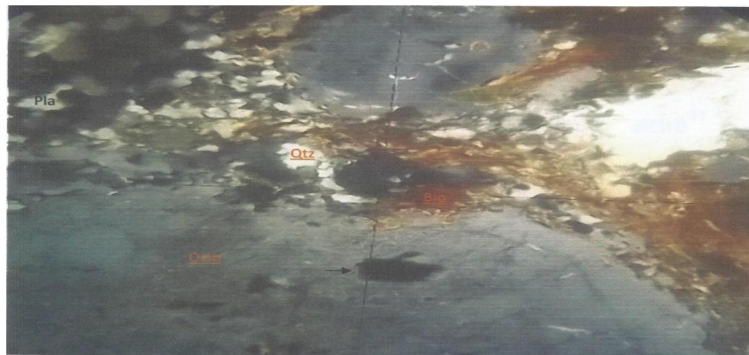
Fig. 11. Photomicrograph of granite, showing phnocryst of orthoclase feldspar displaying zoning as shown by the arrow and the groundmass (XPL view, Mag. X 40)
