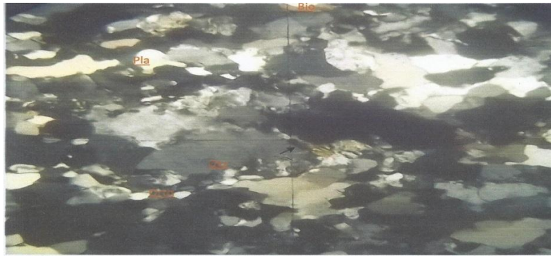
Fig. 9. Photomicrograph of gneiss, showing myrmekitic intergrowth texture of orthoclase crystal and quartz at the cross wires as shown by the arrow (XPL view, Mag. X40)
