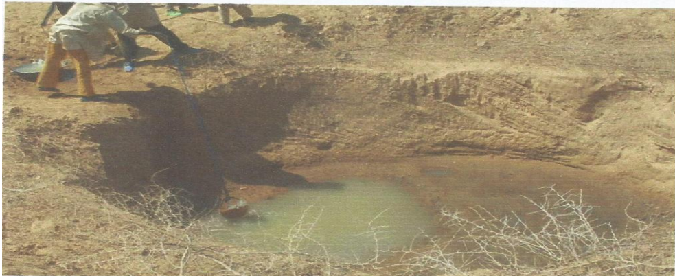
Fig. 15. Field Photography of a hand dug pit along river Yali close to Ungwan Maitokobi with the coordinates latitude 11°37'40.02"N and longitude 007°32'22.07"E, elevation of 616 m and a depth of 1.4 m
