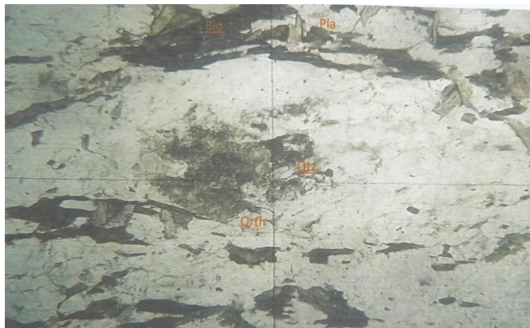
Fig. 8. Photomicrograph of gneiss, shows crystals of orthoclase, biotite and groundmass aligned in a preferred direction (Orth-orthoclase, Bio-biotite, Pla-plagioclase, Qtz-quartz) applicable to all photomicrographs (PPL view, Ma. X40)
