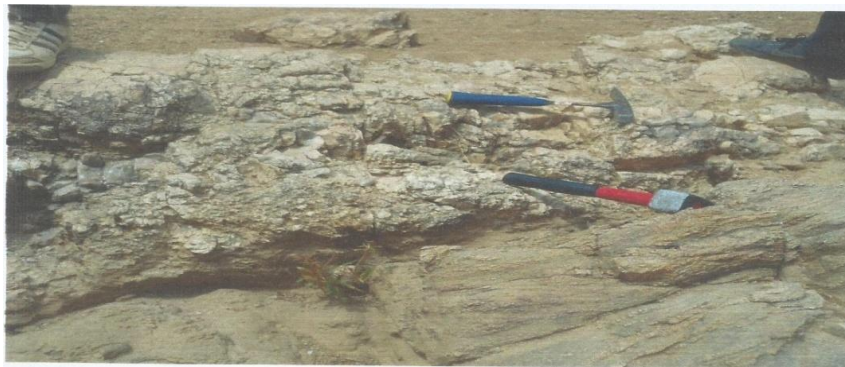
Fig. 7. Field photograph of a pegmatite dyke observed in a weathered gneiss with coordinates latitude 11°37'46.5"N, and longitude 007°32'05.8"E
