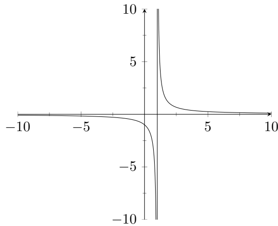
Figure 1: Graph of f(x) = 1/(x - 1)
