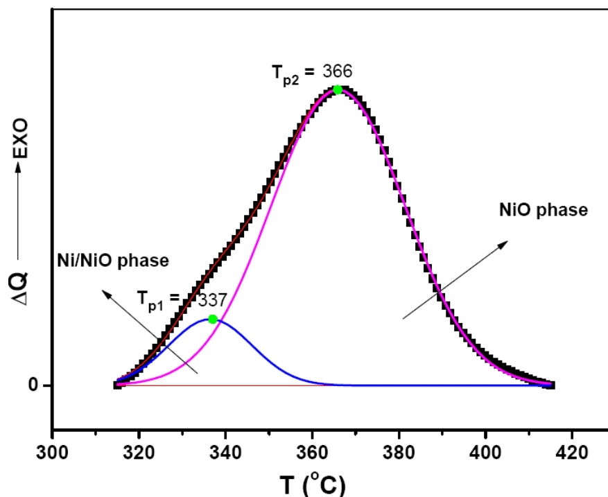
Fig. 2. DSC traces for Ni/NiO and NiO overlapped phases at heating rate 10°K/min
