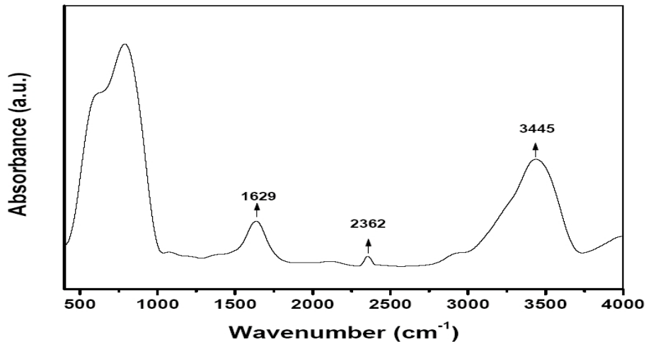
Fig. 6. IR absorbance spectra of NiO nanoparticles
