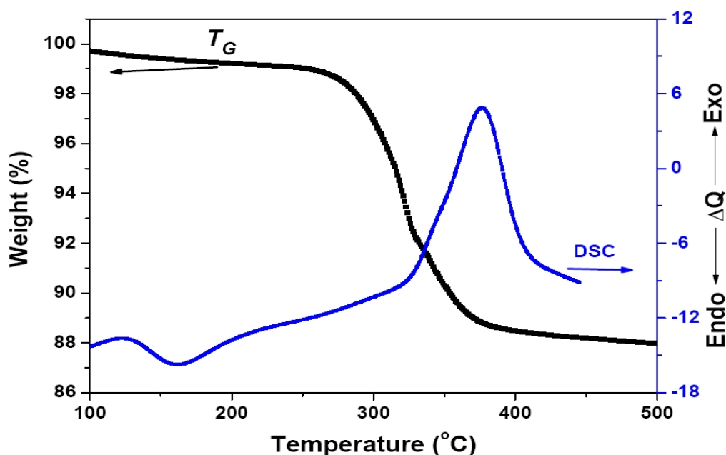
Fig. 1. TGA and DSC curves of the precursor
