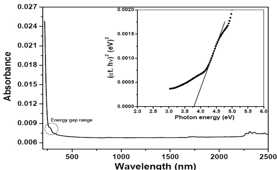
Fig. 7. UV-Vis-NIR absorbance spectrum of Ni/NiO nanoparticles
