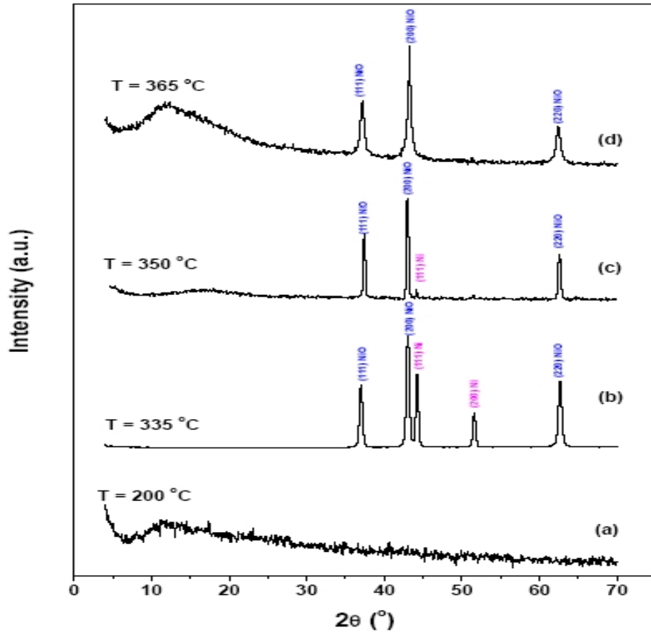
Fig. 3. X-ray diffraction spectra of precursor at different annealing temperatures
