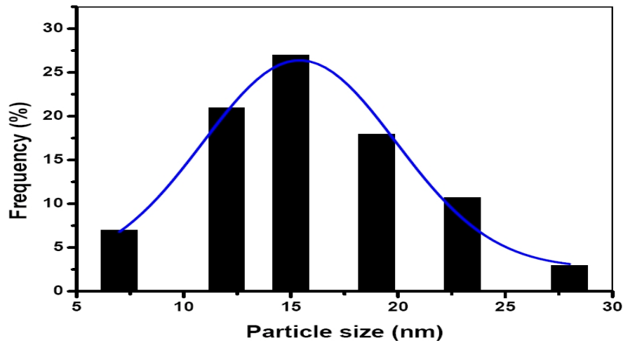
Fig. 5. Particle size distribution of NiO nanoparticles
