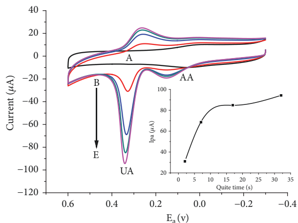
FIGURE 5: Cyclic voltammograms of FeZ-G/GCE pH 7 PBS containing (A) no UA and AA at a quiet time of 2 s (A) and (B-E) containing 1 mM of UA and 1 mM of AA at various quiet times (B-E: 2, 7, 17, and 32 s, respectively).
